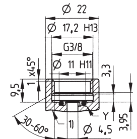
Counter part G 3/8 sealed at front
