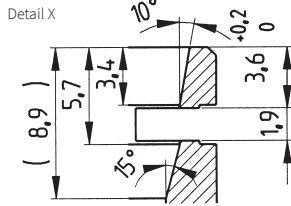
Counter part for plug connector
